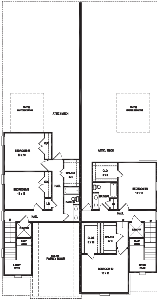
SECOND LEVEL FLOOR PLAN
