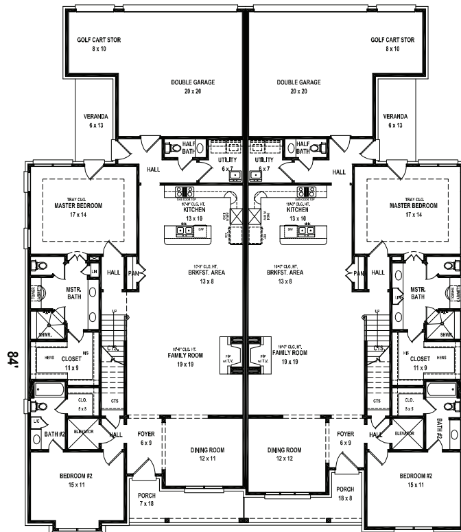
FIRST LEVEL FLOOR PLAN
