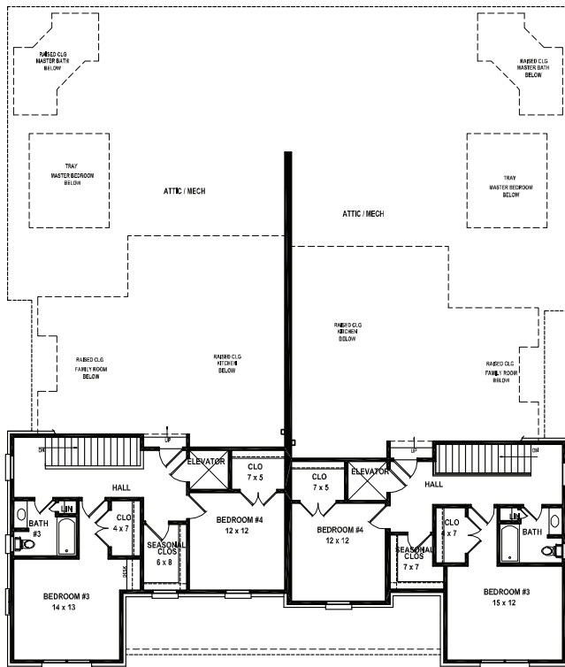
SECOND LEVEL FLOOR PLAN
